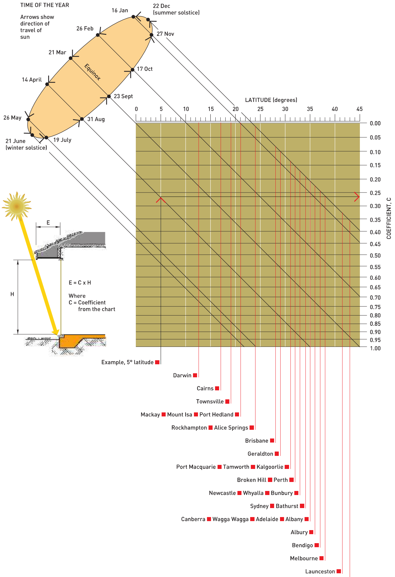
Figure 15 Eaves overhang design chart
